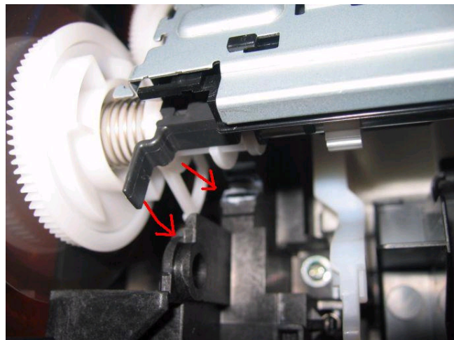
8) Connect the springs on each side of the spur holder to the switch system unit and the purge drive system unit respectively.
