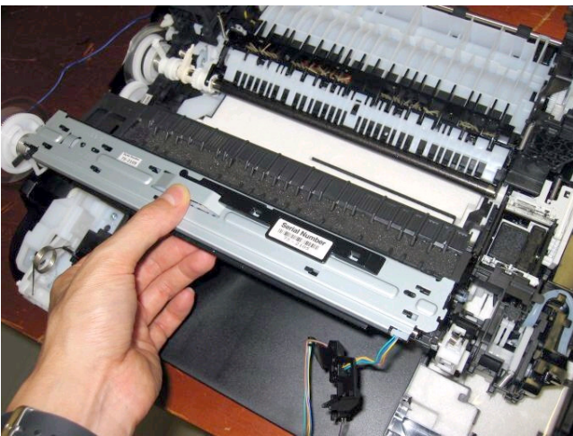
8) Connect the springs on each side of the spur holder to the switch system unit and the purge drive system unit respectively.
